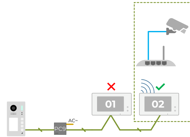
DH470 Wi-Fi to private camera
